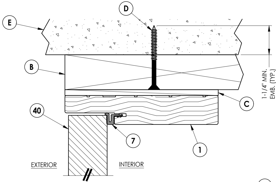
2 VERTICAL CROSS SECTION 3 Outswing shown w/ 2X Buck Installation
