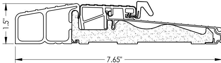
14 OUTSWING BUMP THRESHOLD ENDURA ZOB SERIES w/ 2" Extender
