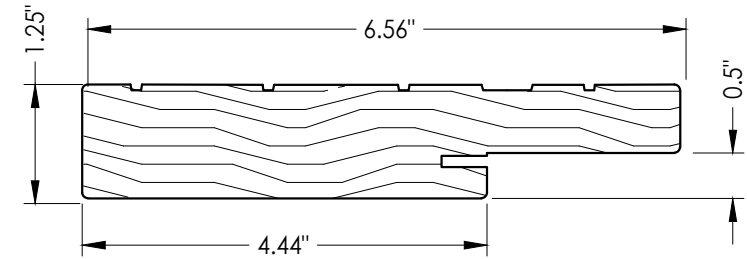
1 WOOD JAMB FINGER JOINT PINE
